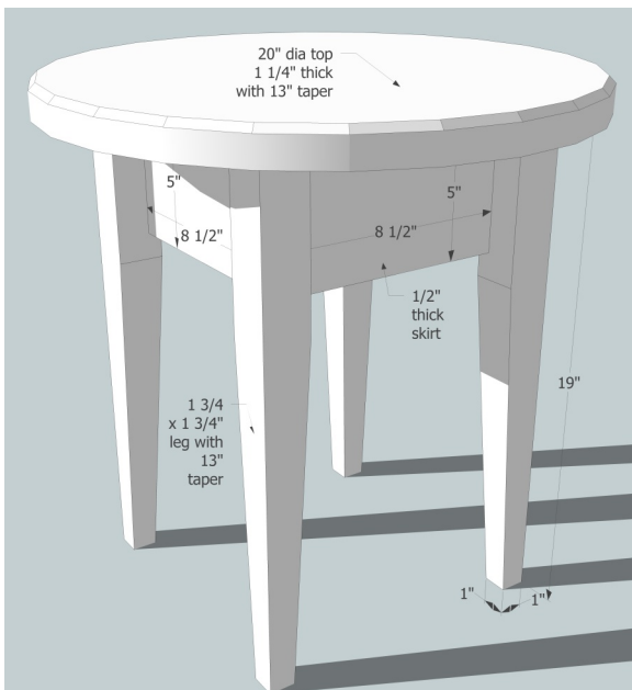
20" diameter table with 5" skirting
