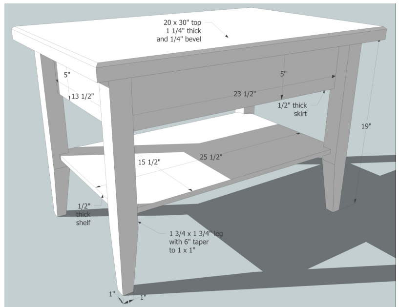
20 x 30" table with 5" skirting and shelf
