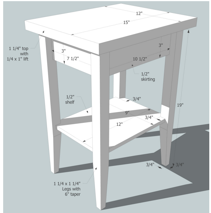
12 x 15" side table with 3" skirting and shelf
