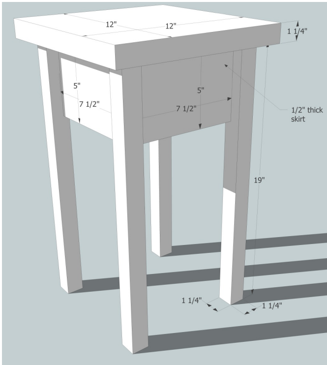
12 x 12" plant stand with 5" skirting
